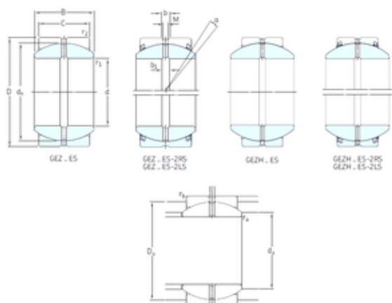
Bearing No. GEZH408ES
