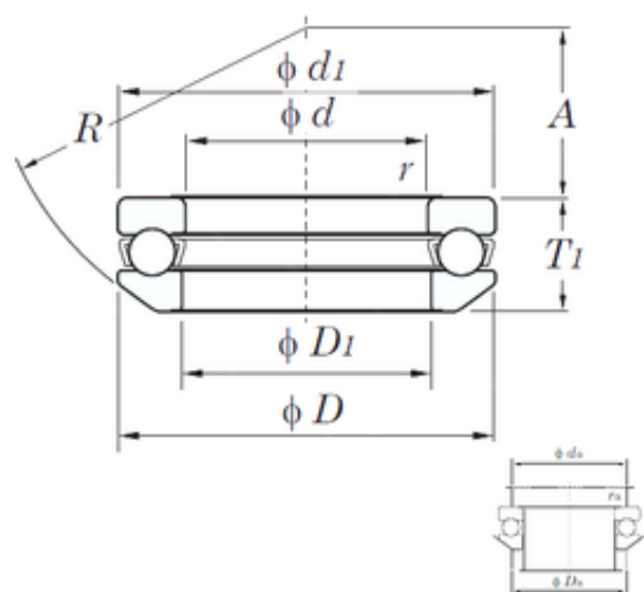
Bearing No. 53244
