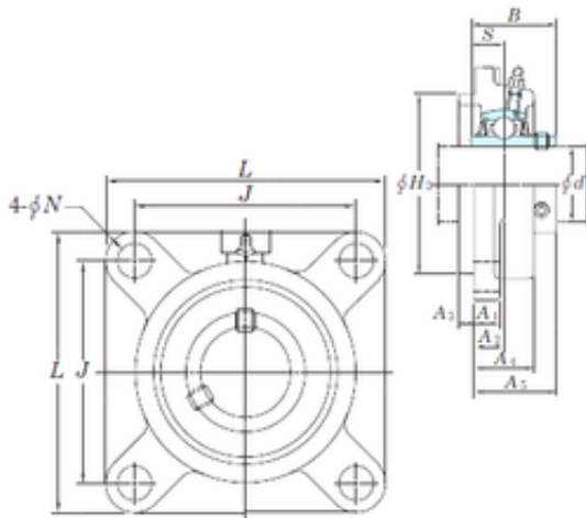
Bearing No. UCFS309-28
