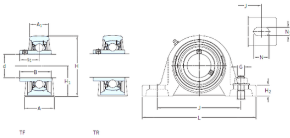
Bearing No. SYJ 1.3/4 TF
