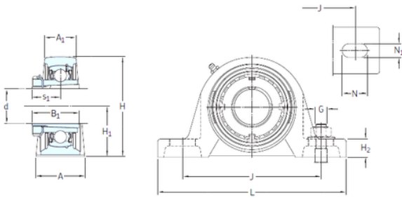
Bearing No. SYJ 50 KF+HE 2310
