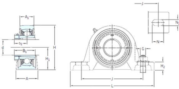
Bearing No. SYJ 50 KF+HS 2310
