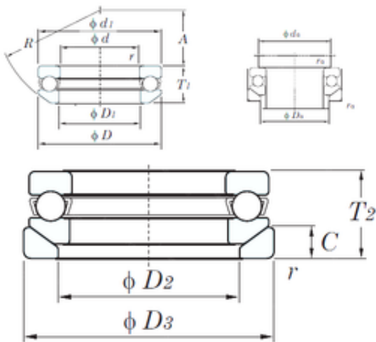
Bearing No. 53320U
