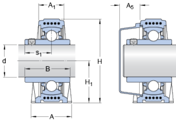
Bearing No. SYK 35 TD
