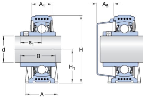
Bearing No. SYK 35 TF
