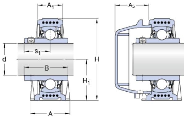
Bearing No. SYWK 25 YTA
