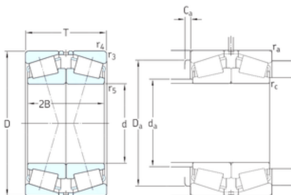
Bearing No. 30238J2/DFC700
