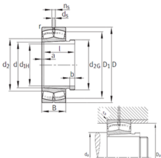
Bearing No. 23240-B-K-MB+AH3240
