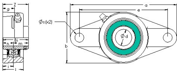
Bearing No. UCFL 205
