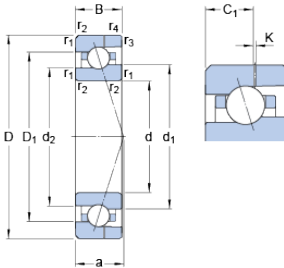
Bearing No. 7002 CE/HCP4AH
