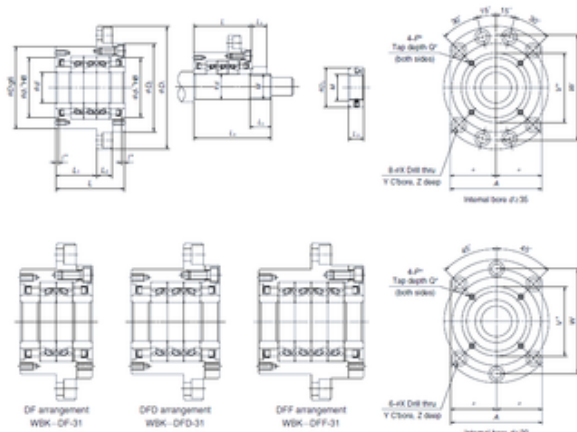
Bearing No. WBK40DFD-31
