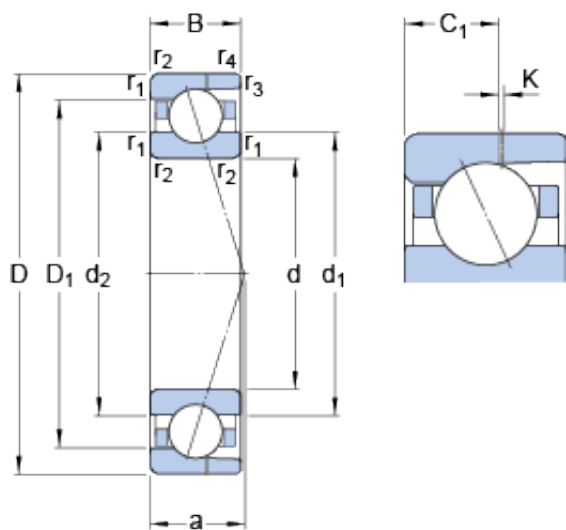
Bearing No. 7003 ACD/P4AH
