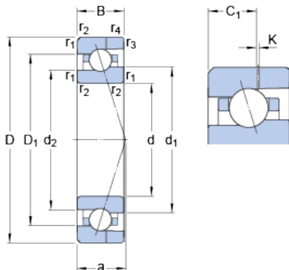
Bearing No. 7003 ACE/P4AH
