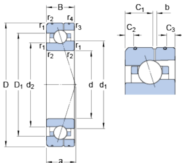
Bearing No. 7004 ACE/P4AL
