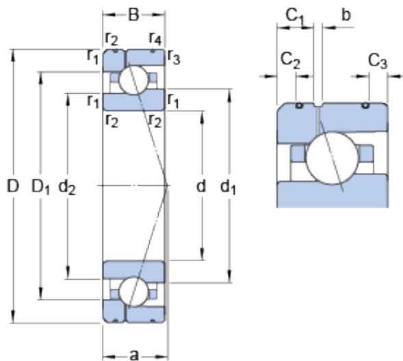
Bearing No. 7004 ACE/P4AL1
