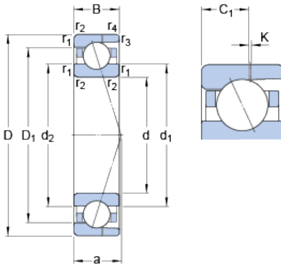
Bearing No. 7004 CD/P4AH
