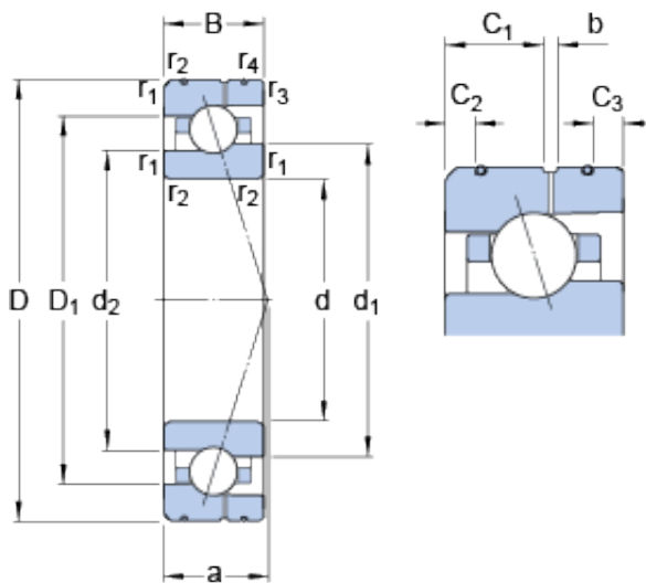
Bearing No. 7005 ACE/P4AL
