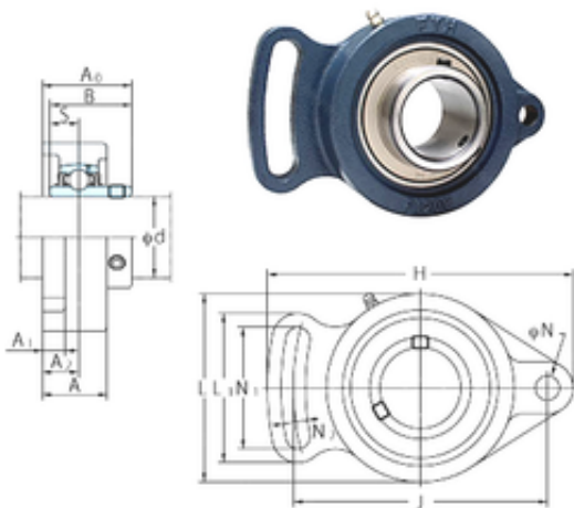
Bearing No. UCFA210
