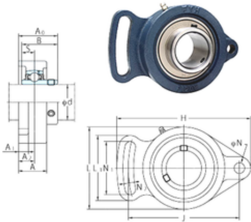
Bearing No. UCFA205-15
